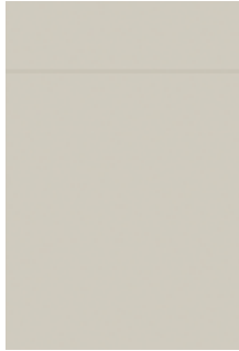
Clay
