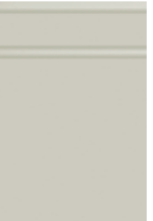
Limestone
